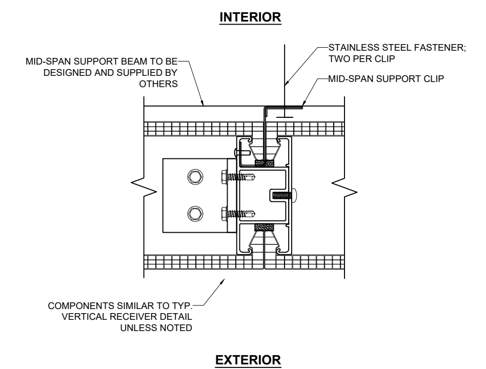
H 1 MID-SPAN SUPPORT FOR TALL SPANS SCALE: 3/8" = 1"
