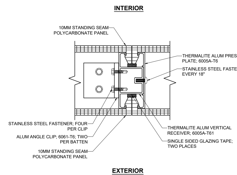
G 1 TYP. VERTICAL RECEIVER SCALE: 3/8" = 1"
