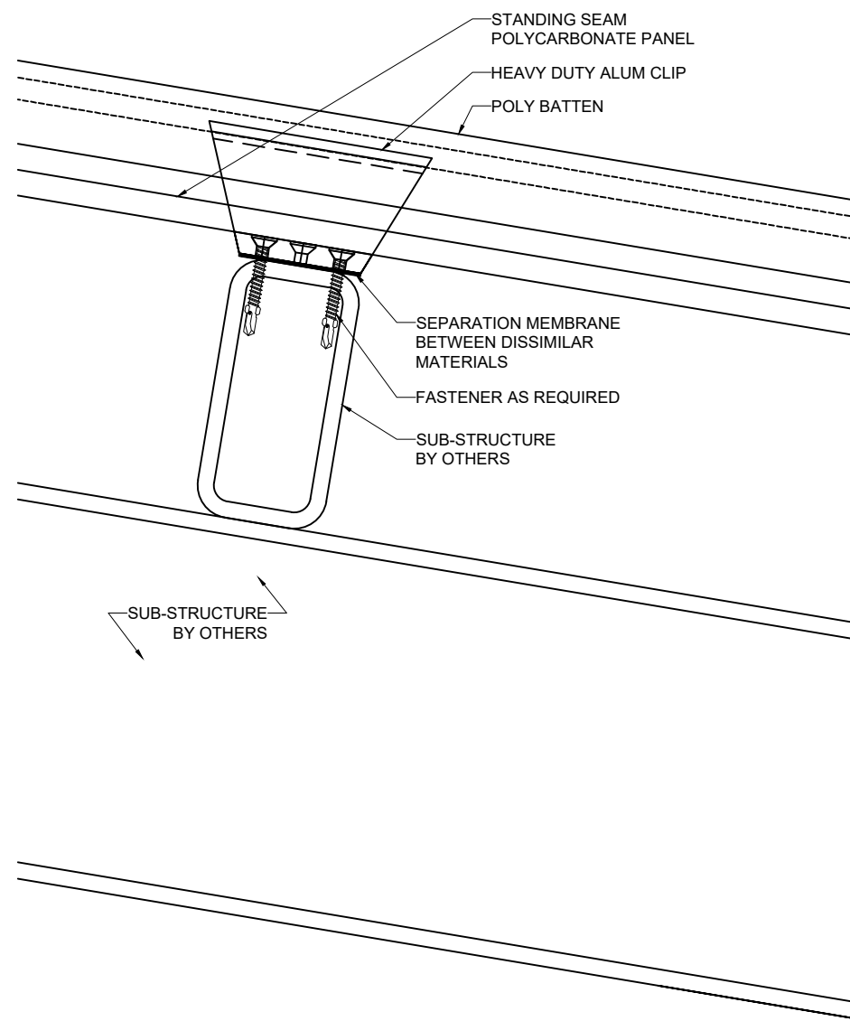
D 1 TYP. MID-SPAN SCALE: 3/8" = 1"
