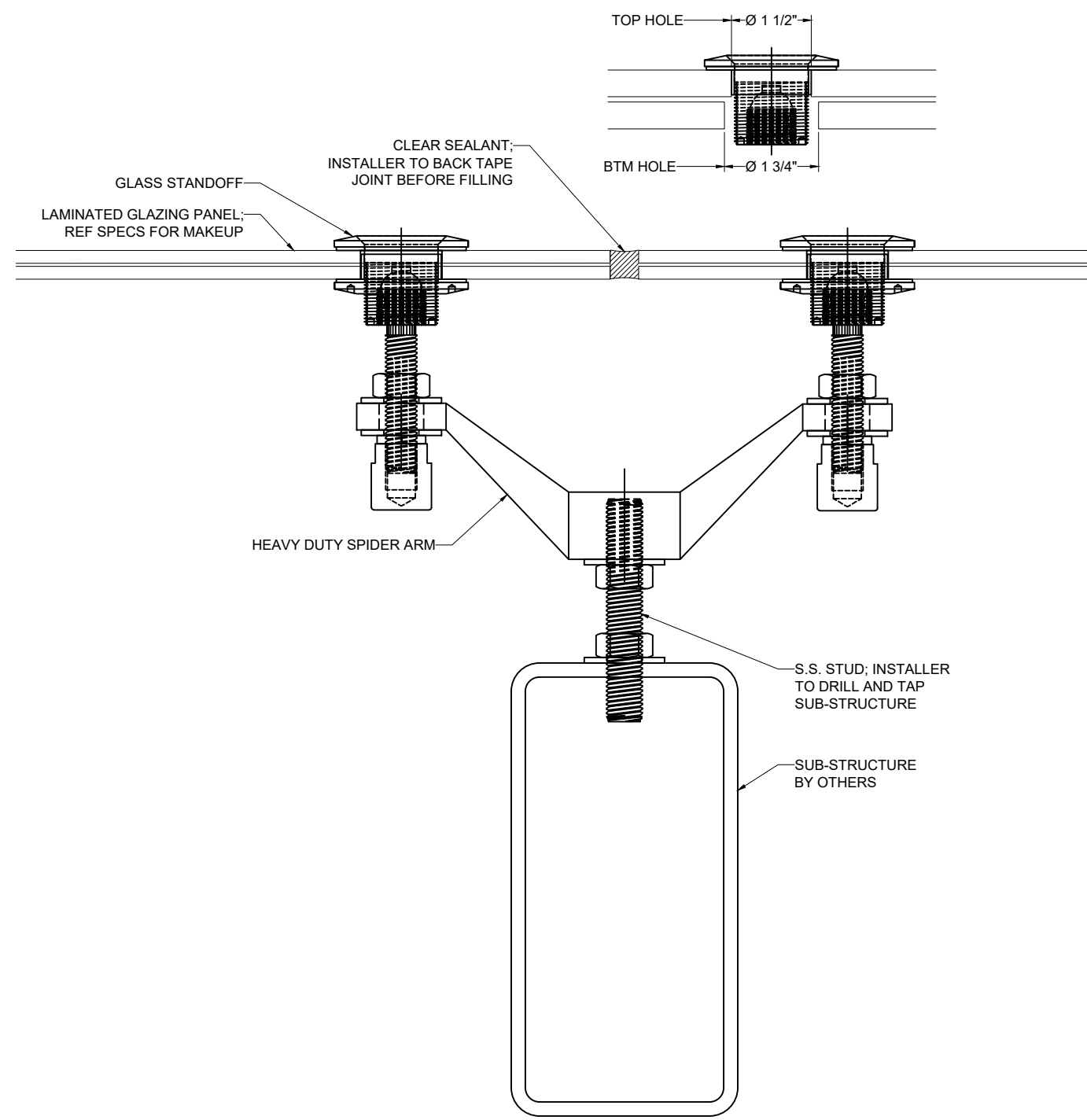
D 1 TYP. PURLIN SCALE: 3/8" = 1"
