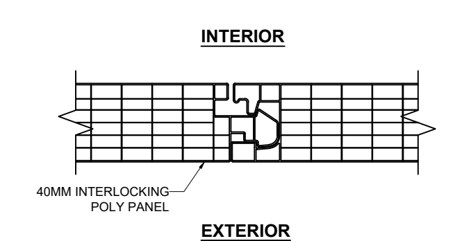
G 1 TYP. PANEL JOINT SCALE: 3/8" = 1"
