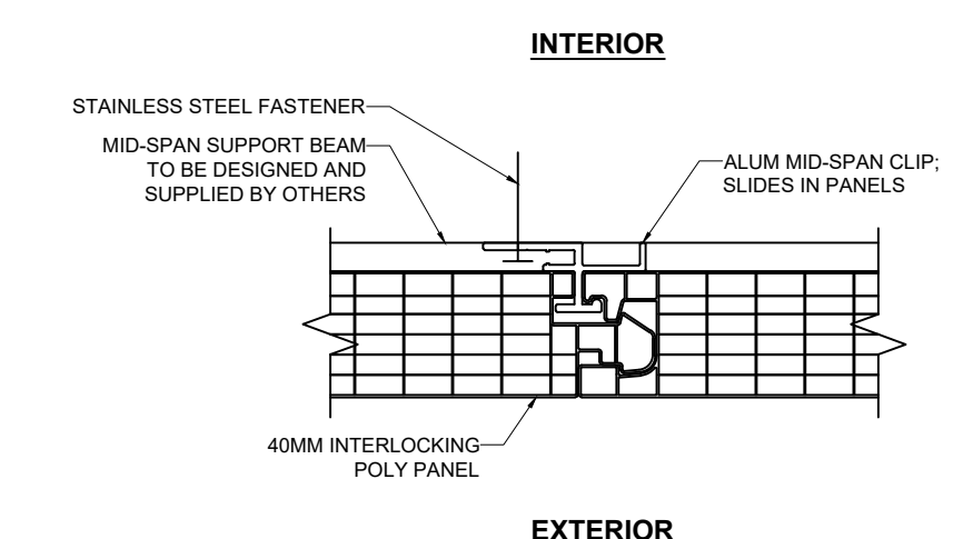
H 1 PANEL JOINT @ MID-SPAN SCALE: 3/8" = 1"
