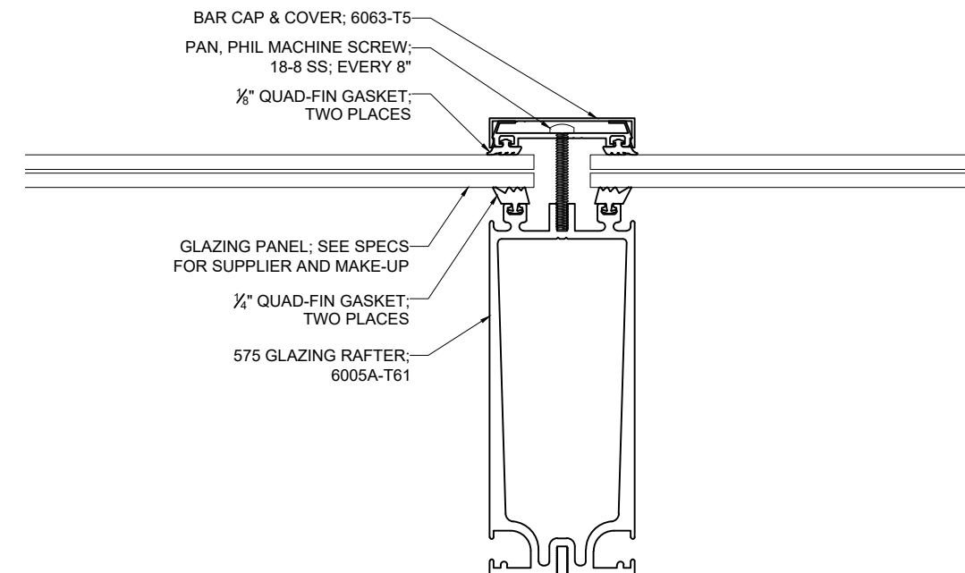
F 1 TYP. RAFTER SCALE: 3/8" = 1"
