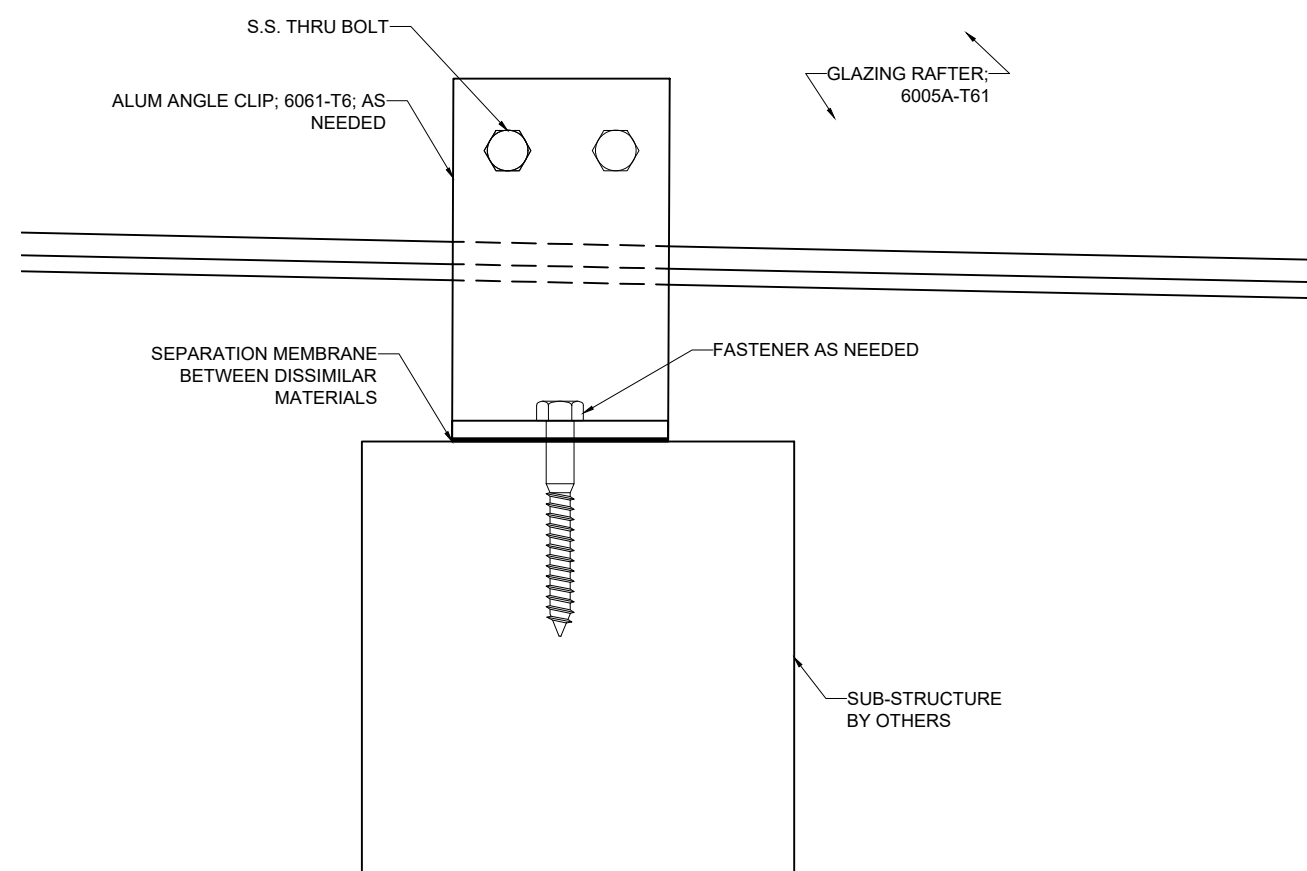
C 1 MID-SPAN SUPPORT SCALE: 3/8" = 1"
