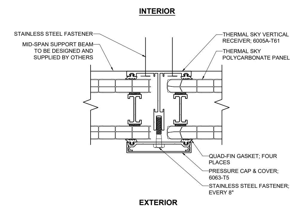
H 1 MID-SPAN SUPPORT SCALE: 3/8" = 1"
