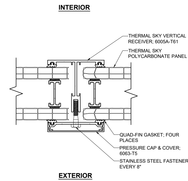
G 1 TYP. INTERMEDIATE SCALE: 3/8" = 1"
