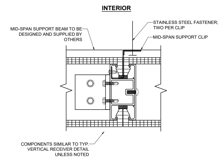
H 1 MID-SPAN SUPPORT FOR TALL SPANS SCALE: 3/8" = 1"
