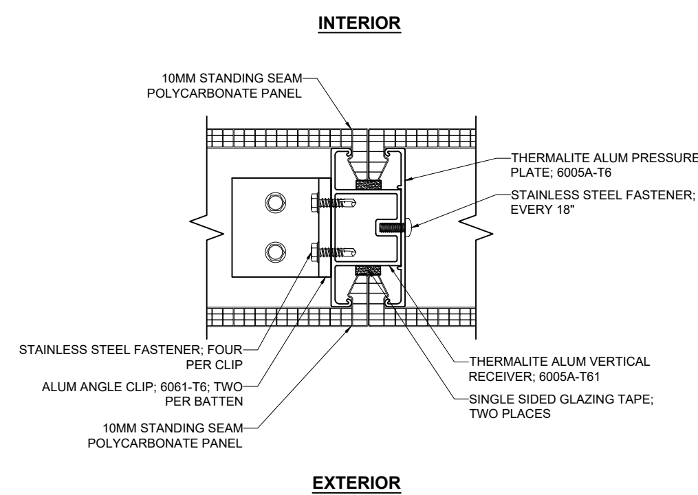
G 1 TYP. VERTICAL RECEIVER SCALE: 3/8" = 1"
